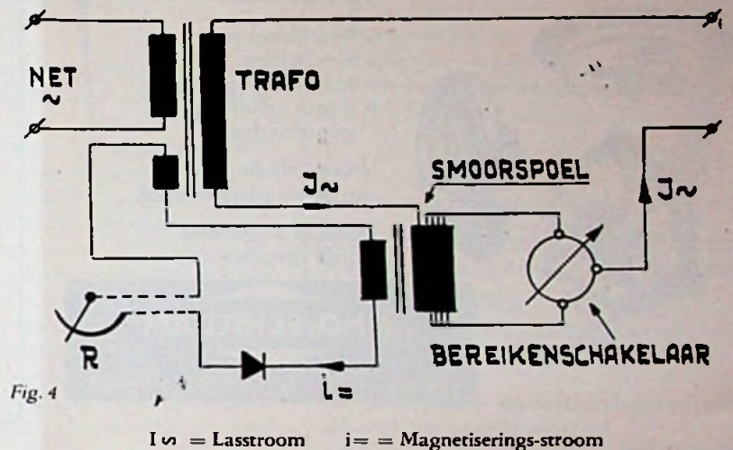
Lastransformator type ML35
